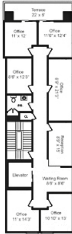
Third Floor
